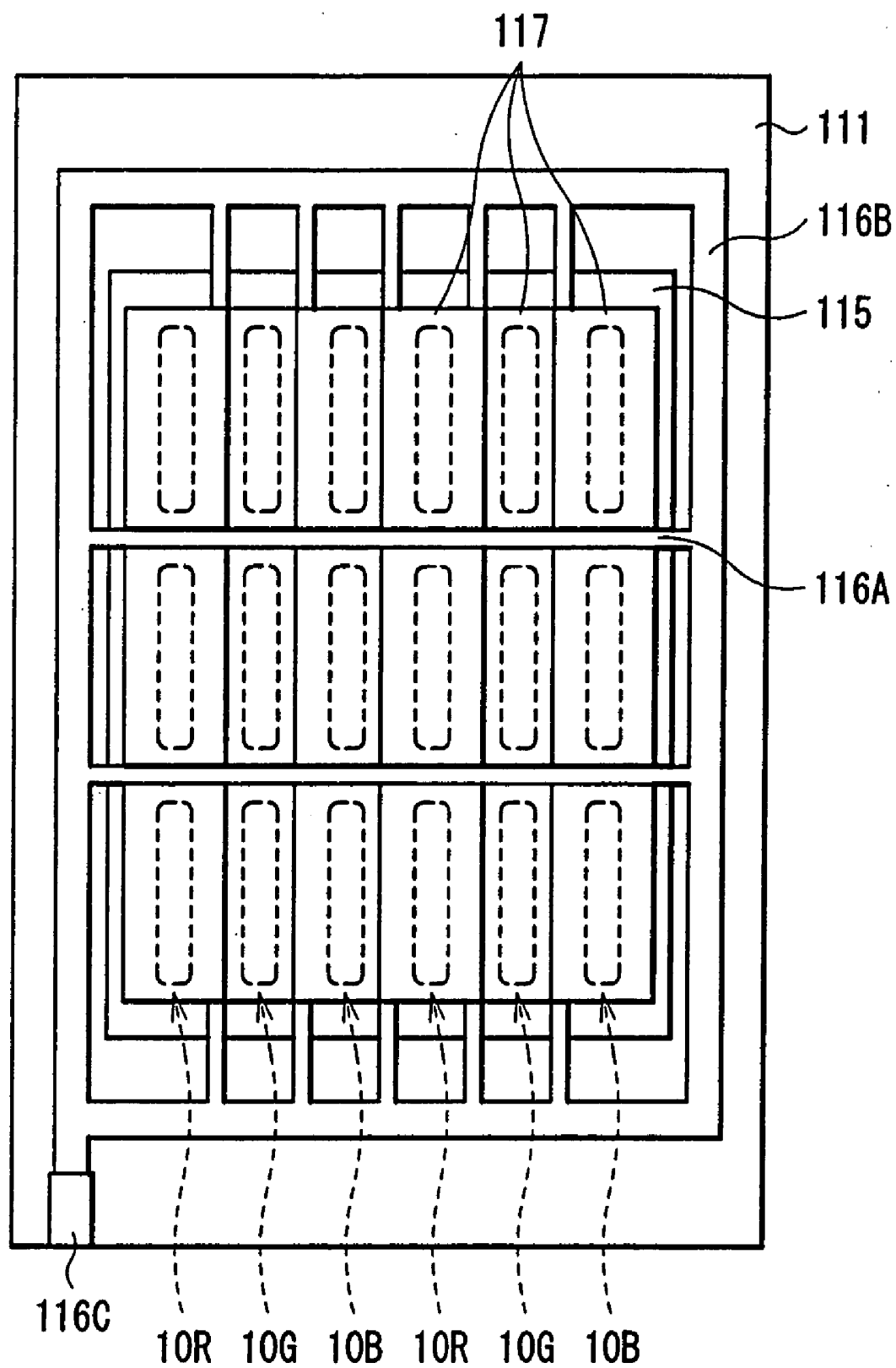
FIG. 6 PRIOR ART
